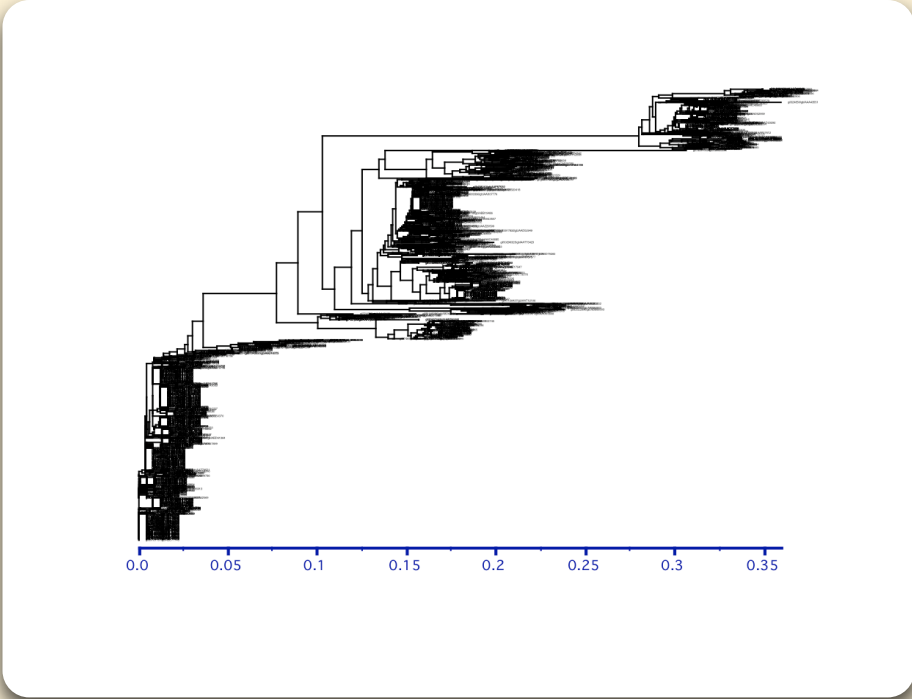
Figure 4. Influenza A virus NS1 full length protein sequences aligned using the MUSCL program and subsequently order as a phylogenetic tree using CLUSTALW. The results of the single-linkage clustering determined there are 6 NS1 clades in the Influenza samples.
